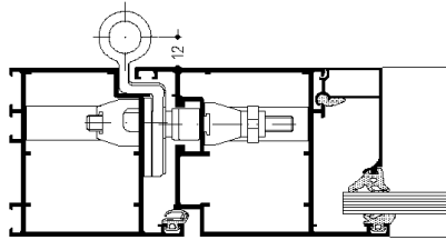
Aluminium Rollenband WICONA
