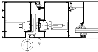
Aluminium Rollenband WICONA
