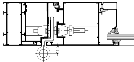
Aluminium Rollenband WICONA
