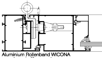
Aluminium Rollenband WICONA
